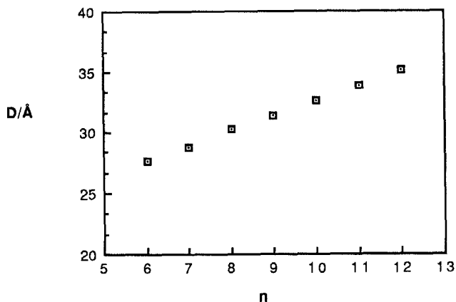
Figure 8. Intercolumnar distance as a function of n for compounds 1 and 2 .
